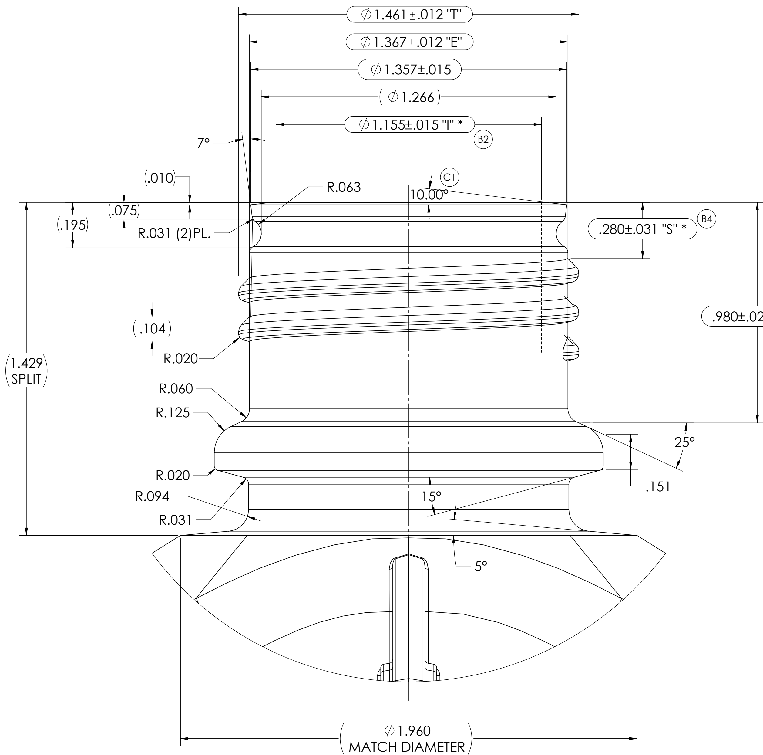
DETAIL A SCALE 4 : 1
